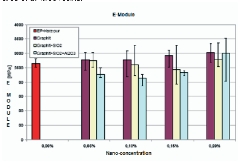
Fig.12: Comparison of E-Modules
