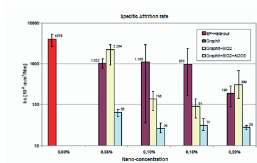
Fig. 8 Comparison of the specific attrition rates
