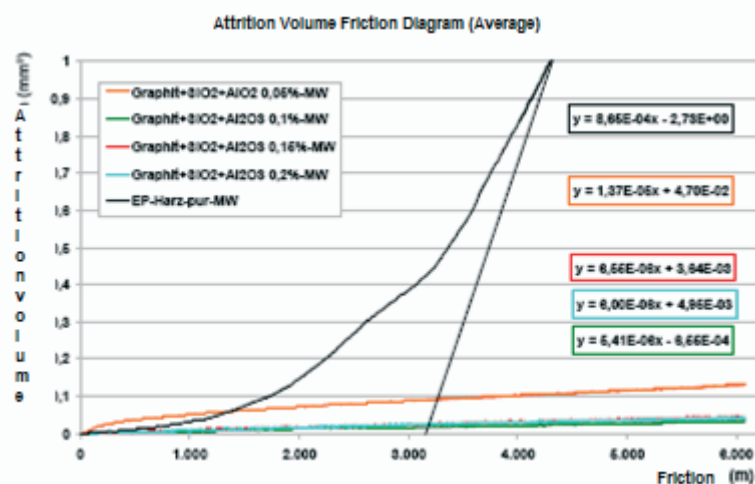
Fig.6: Attrition volume of ER-resin with different concentrations of graphite/SiO 2 /Al 2 O 3
