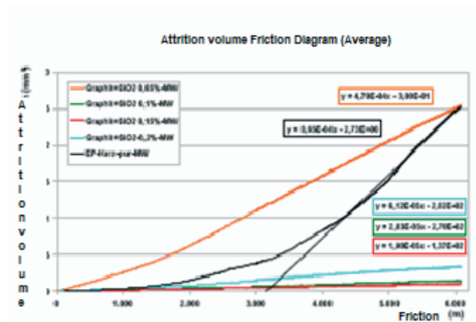
Fig.5 Attrition Volume of ER- resin with different concentrations of the mixture of graphite and SiO 2
