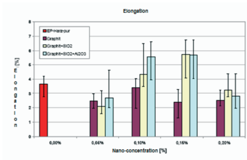
Fig. 11: Comparison of Elongation
