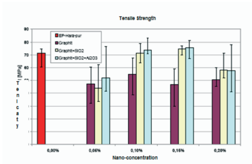
Fig. 10: Comparison of tensile strength
