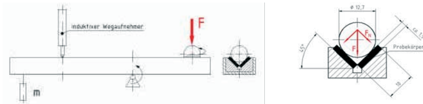
Fig.3 Function of the ball-shaped prism tribometer, Prism open angle 90° as well as arrangements of ball and prism.
