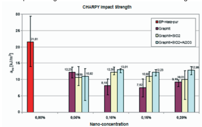
Fig.9 Comparison of CHARPY Impact Strength
