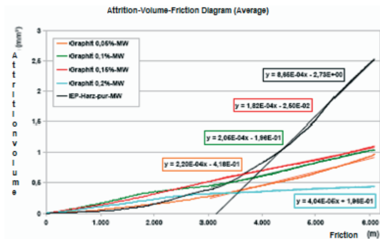
Fig. 4 Attrition volume friction way of ER resin with different graphite concentrations vs. X5CrNi18-10
