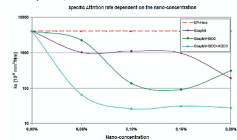
Fig.7: Impacts of the matter concentration on the different attrition rates
